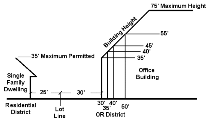
Maximum Building Height Calculation
