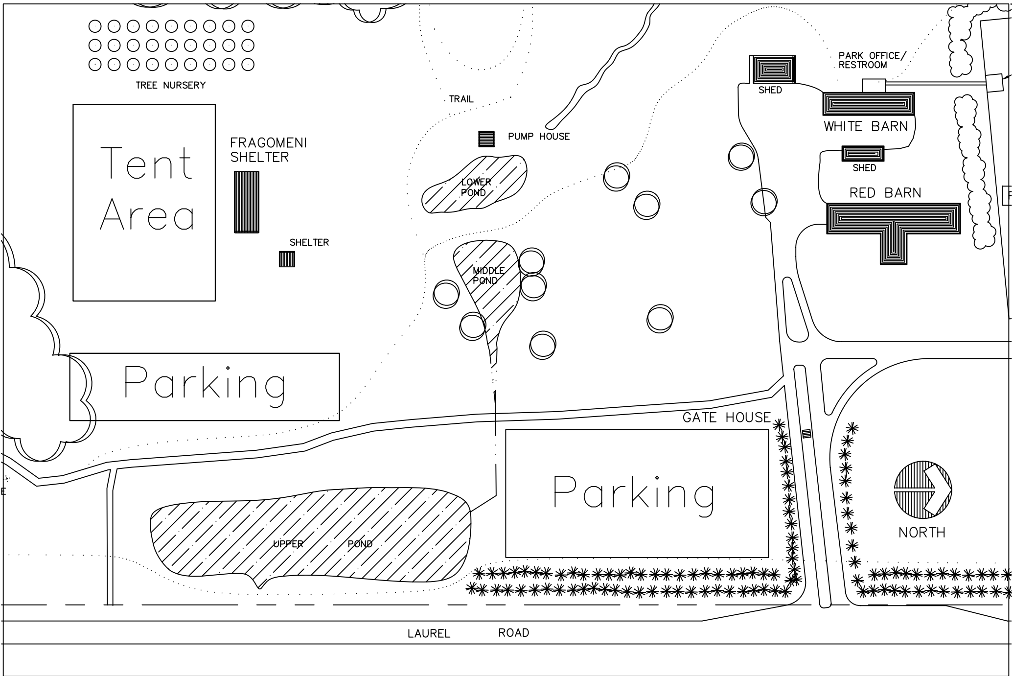
SITE PLAN
